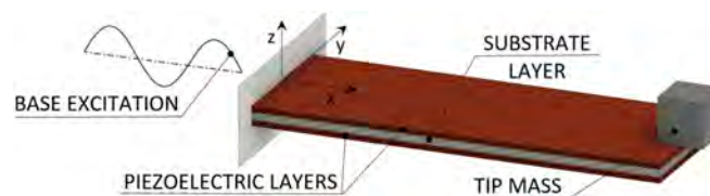
Figure 6. Piezoelectric bimorph vibration EH device [32].
