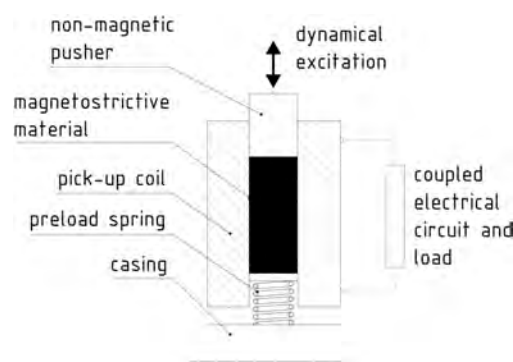
Figure 14. Typical magnetostrictive EH device.
