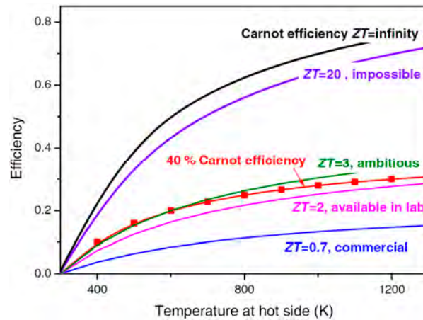
Figure 20. Conversion efficiency of TE materials vs. \Delta T (for T_{cold} = 300K ) and ZT [148]-reprinted by permission from Springer Nature.
