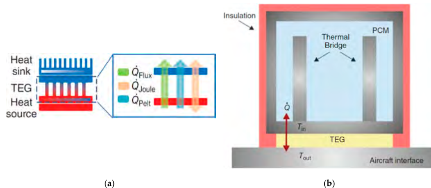
Figure 25. Static (a) and dynamic (b) TEG configurations used in airplanes' fuselages [150].
